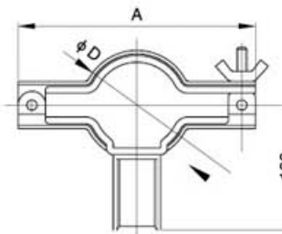
六角型管支架带柄 Hexagon pipe holder with handle 3181017
