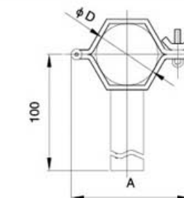
六角型管支架带柄 Hexagon pipe holder with handle 3181018
