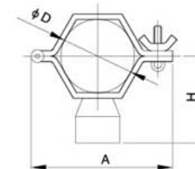
六角型管支架带柄 Hexagon pipe holder with handle 3181018
