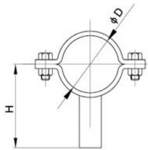
六角型管支架 Hexagon pipe holder 3180013
