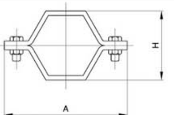
六角型管支架 Hexagon pipe holder 3180014
