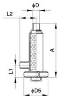
焊接角式过滤器 Welded angle-type strainer | DIN | 3131003
