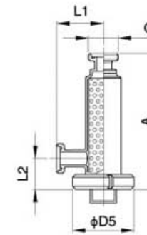
螺纹角式过滤器 Threaded angle-type strainer | DIN | 3133004
