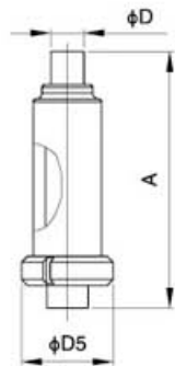
焊接式直通过滤器 Welded straight strainer | DIN | 3131001
